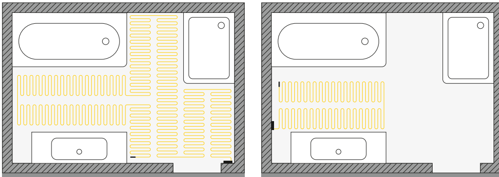
■ BLANKE ELOTOP+ LAID OVER THE WHOLE SURFACE ■ BLANKE ELOTOP+ LAID IN PART OF SURFACE AREA
